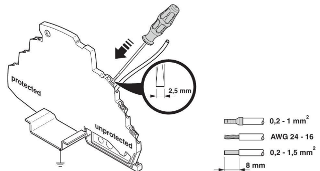
Figure 11 Connection version Push-in connection (overall width 3.5 mm)
