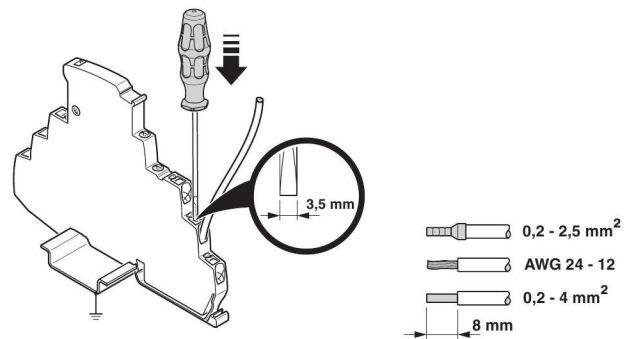
Figure 10 Connection version Push-in connection (overall width 6 mm)
